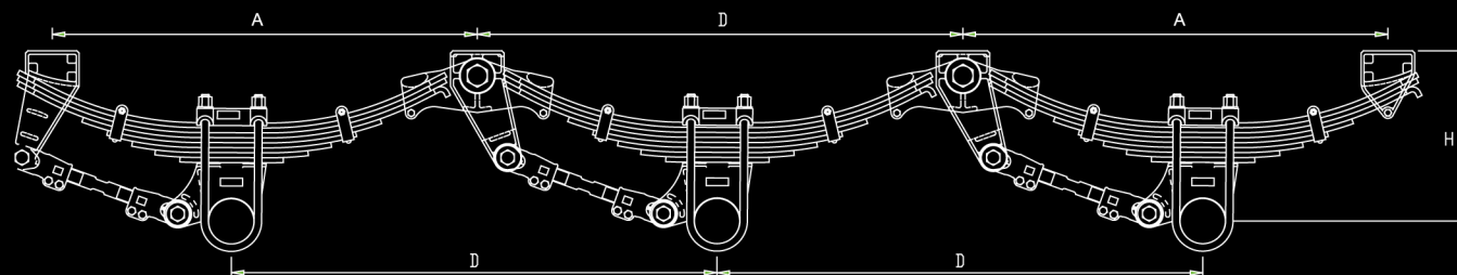
TRI AXLE
